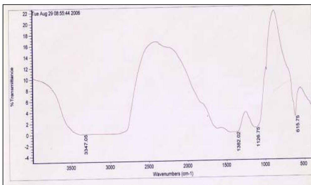
Figure 3: FTIR Spectra of solid glucosamine sulphate (Test)
