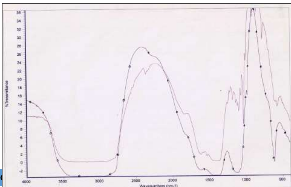
Figure 3: FTIR Spectra of solid glucosamine sulphate (Test)
