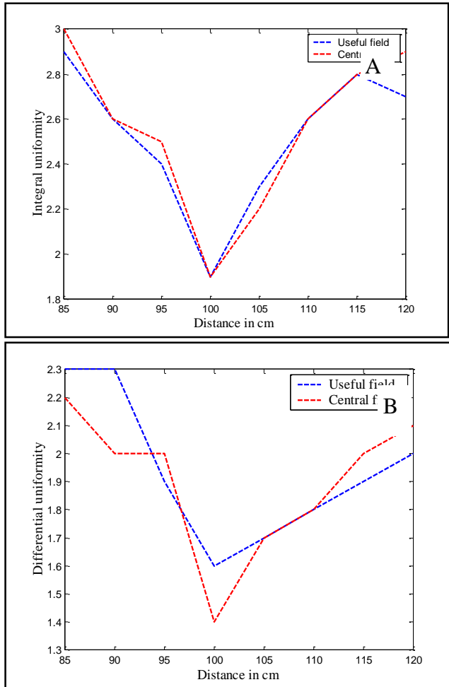
Fig. 1: Intrinsic uniformity versus source-to-camera distance, (A) distance versus integral uniformity (B) distance versus differential uniformity. The best values of intrinsic uniformity were at a distance of 100 cm.
