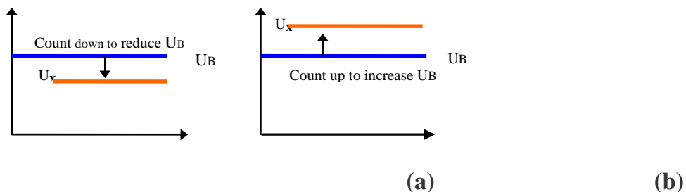
Fig.2. Counting procedure of the tracking ADC. (a) U_x < U_B , (b) U_x > U_B .
